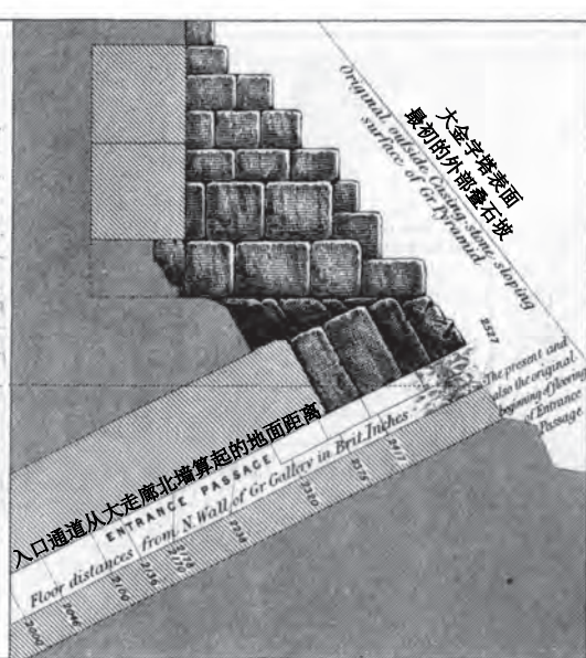
垂直纵剖面 VERTICAL LONGITUDINAL SECTION. 向西看 Looking West. OF THE UPPER, NORTH, END, OR BEGINNING, OF THE ENTRANCE PASSAGE 从北部顶端或入口处 INTO GREAT PYRAMID 进入大金字塔
